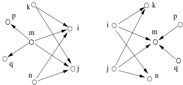
Figure 2: Importance of hyperlink weight normalization.
